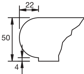
Typical 50mm bullnose Section
