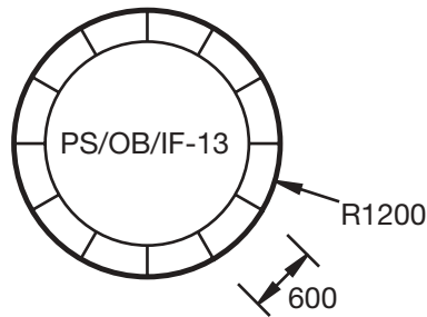
Internal Bullnose
