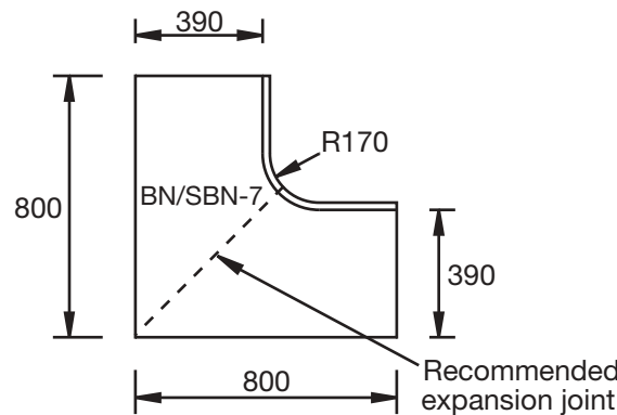
Internal corner stone - round
