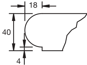
Typical 40mm bullnose Section
