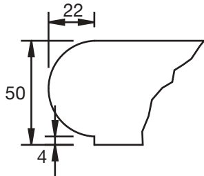
Typical 50mm bullnose Section
