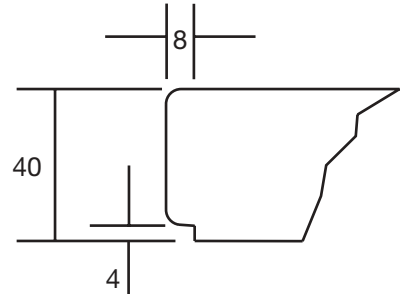
Typical 40mm Square Edge Coping Section
