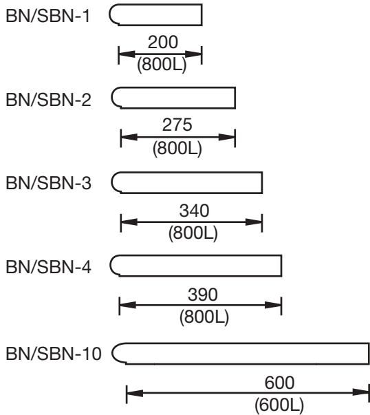
Typical 50mm bullnose Section
